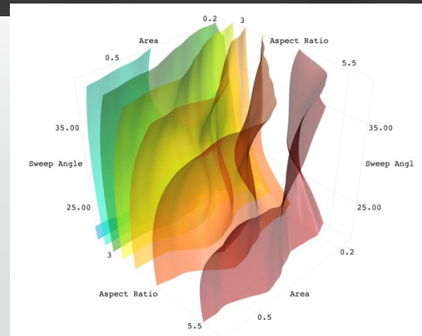
Digital aircraft performance models mapped to the parametric geometries
